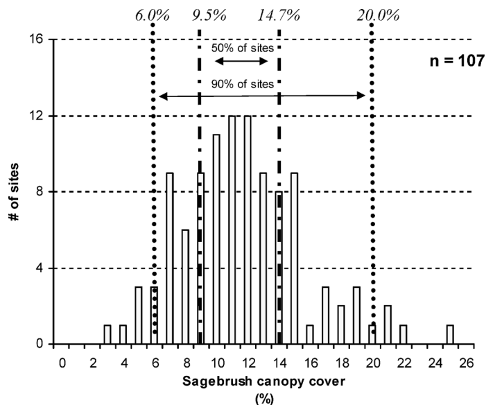
Figure 3. The number of Wyoming big sagebrush sites that produced a given quantity of sagebrush cover. The area between the dotted lines contains the cover values for 90% of the sites. The area between the dashed lines contains the cover values for 50% of the sites.
